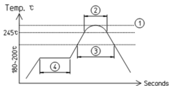
Fig 2. Reflow Profile
