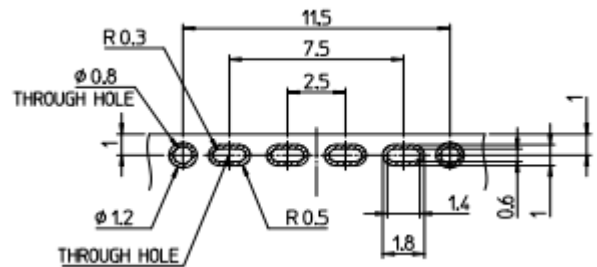
REFERENCE LAND PATTERN
