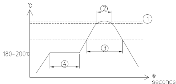
Fig2. Reflow Profile
