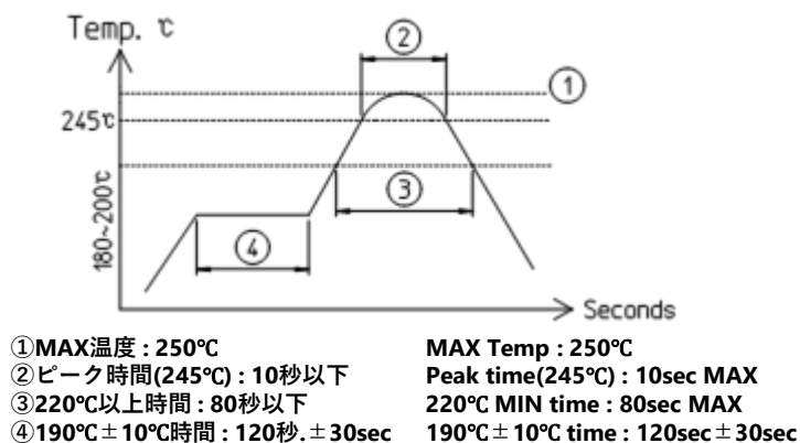
Fig2. Reflow Profile
