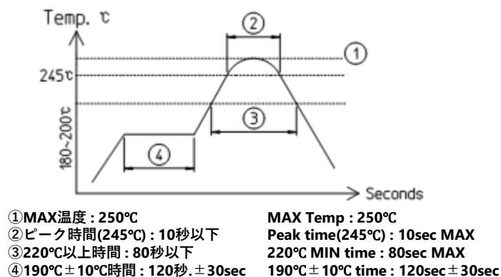
Fig2. Reflow Profile
