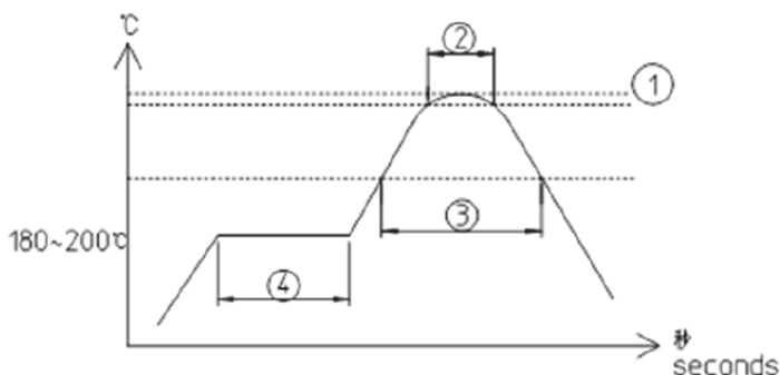
Fig2. Reflow Profile
