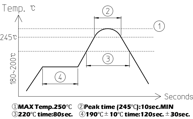
Fig 2. Reflow Profile
